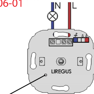
"microswitch" mygtukas
